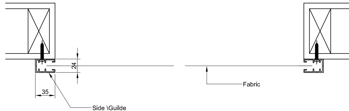
FACE FIXING
