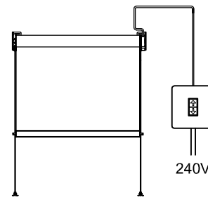
Single Switch
